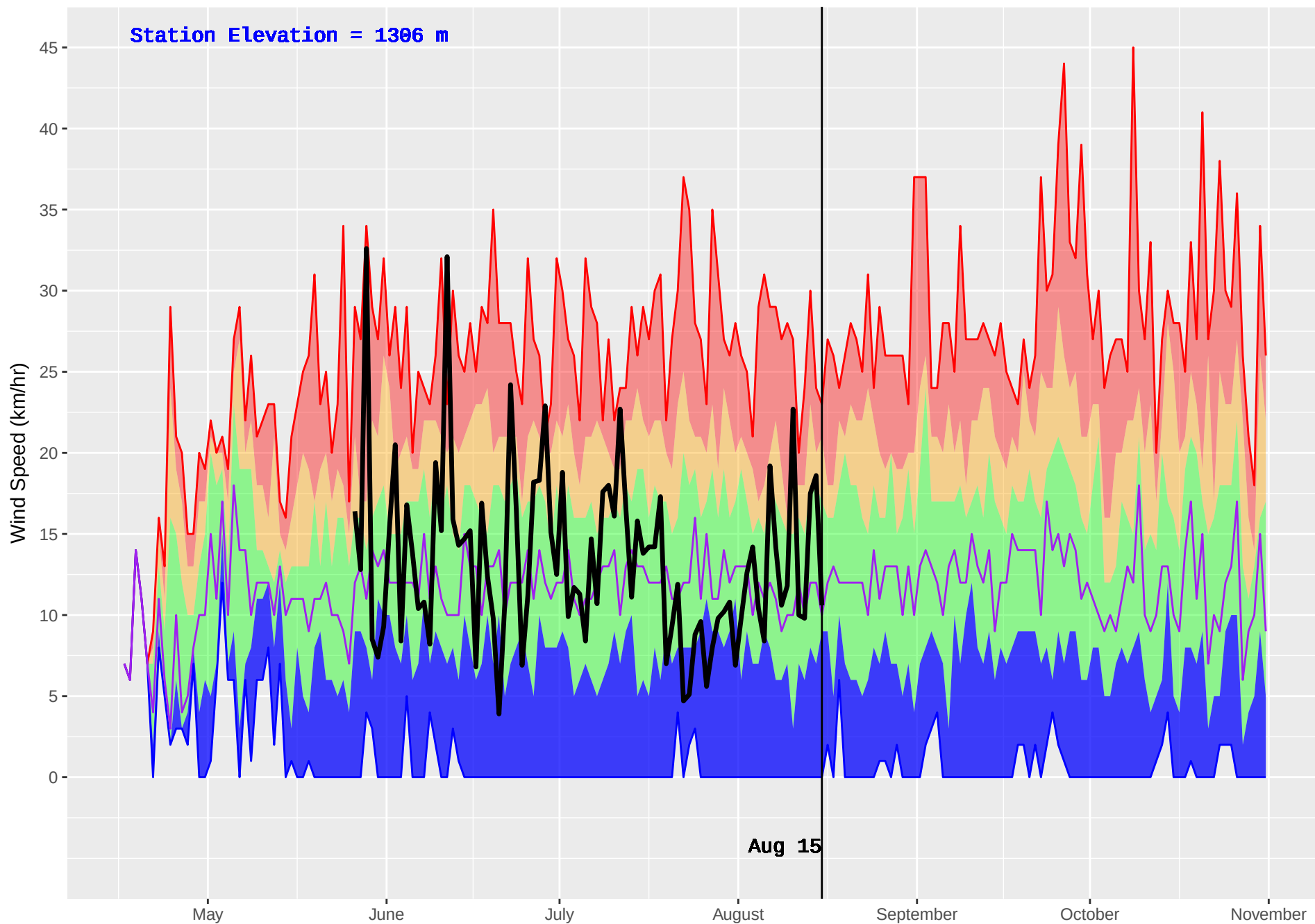
RED DEER (138) : Historical (1988–2016) and Current (2018) Daily Wind Speed
