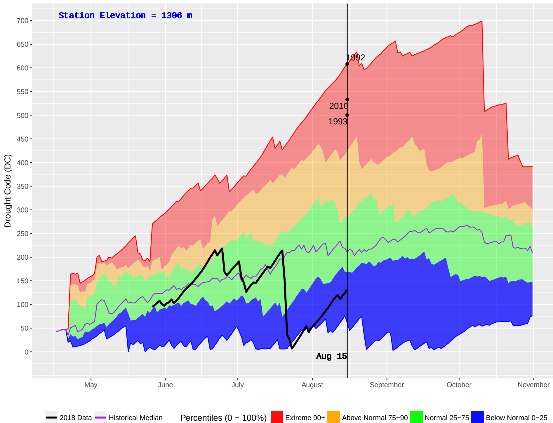
RED DEER (138) : Historical (1988–2016) and Current (2018) Daily Drought Code (DC)
