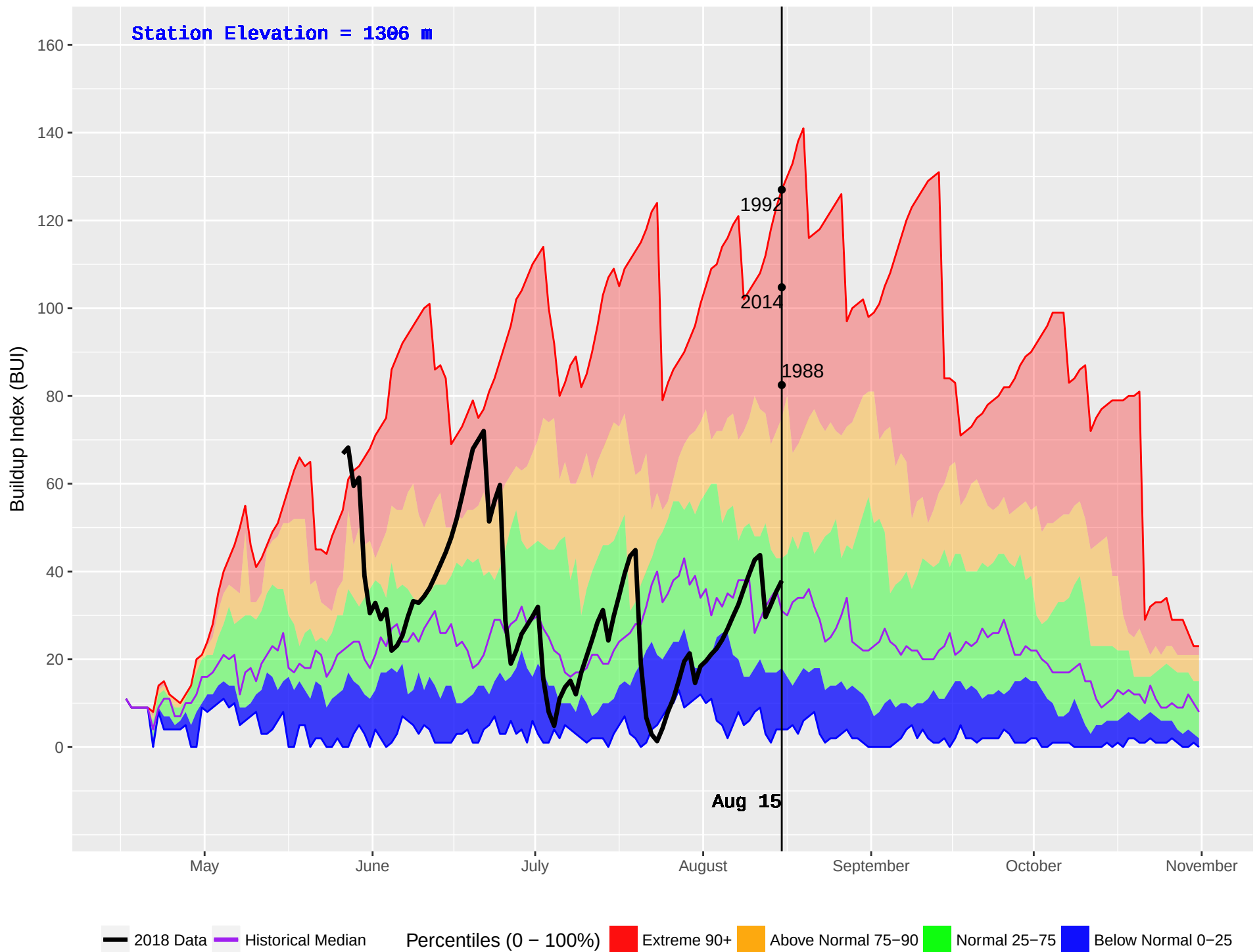
RED DEER (138) : Historical (1988–2016) and Current (2018) Daily Buildup Index (BUI)
