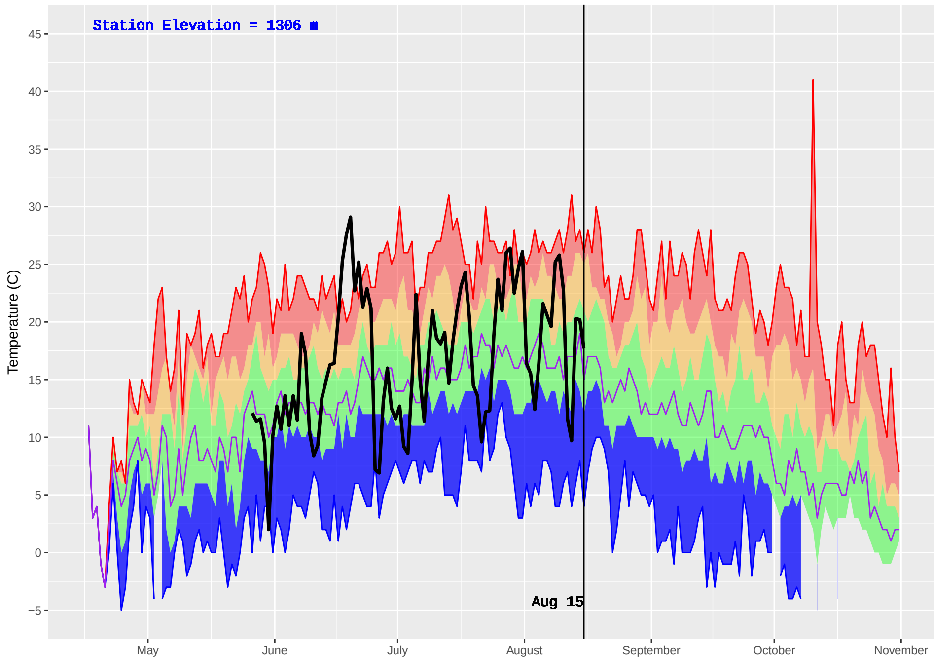
RED DEER (138) : Historical (1988–2016) and Current (2018) Daily Temperature
